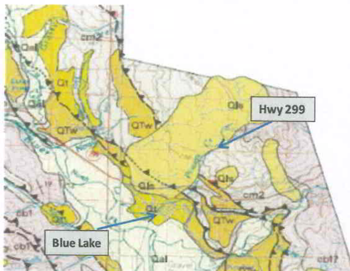
Figure 4 – Portion of Geologic Map near Blue Lake
